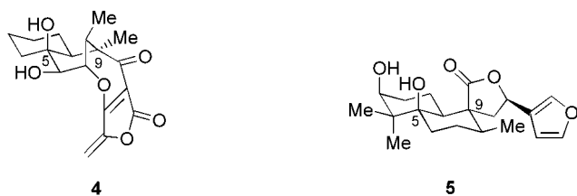
Figure 1. Structure of tetrodecamycin ( 4 ) and dihydroxychiolide ( 5 ).
